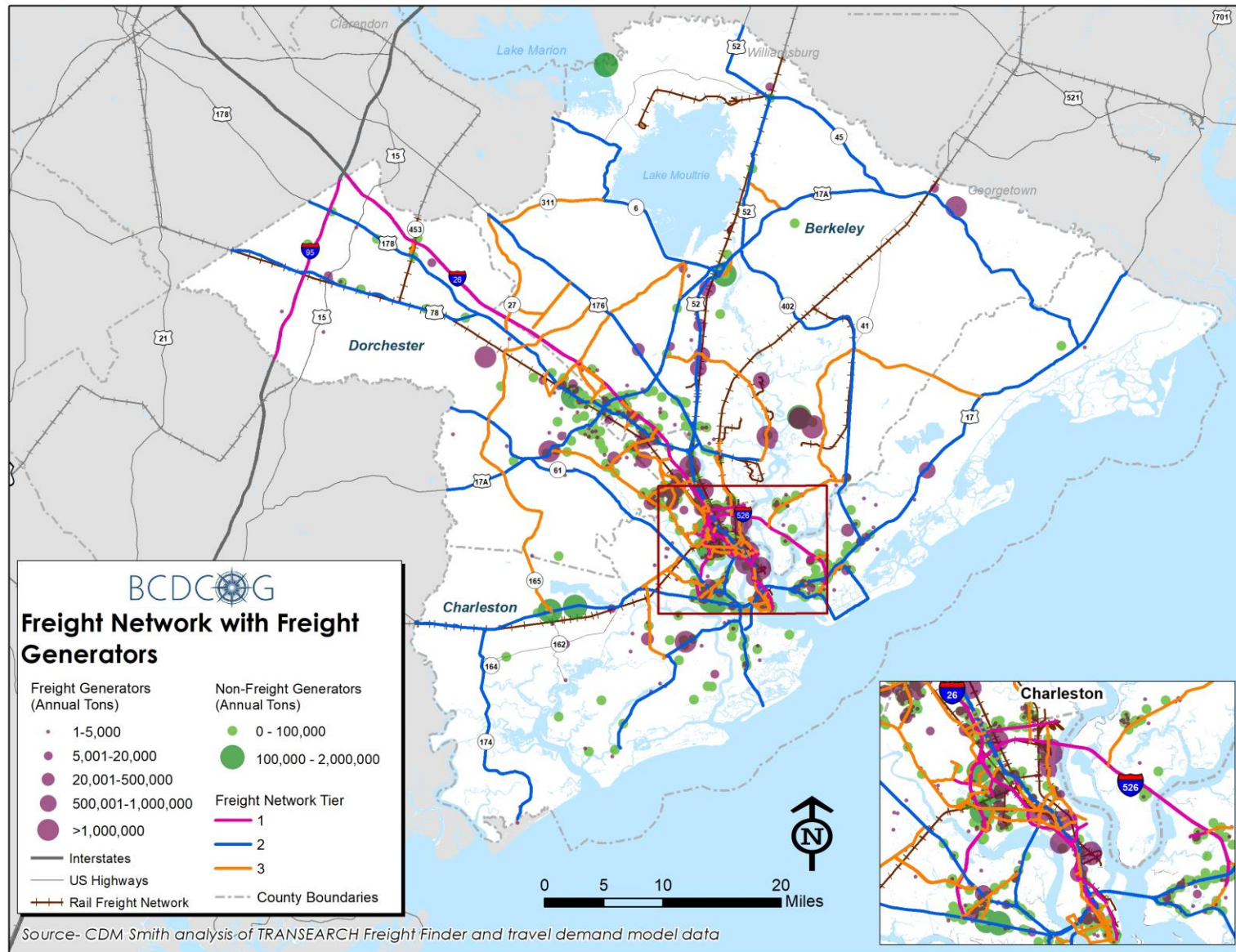
Figure 3-3: BCD Regional Freight Network with Freight Generators
