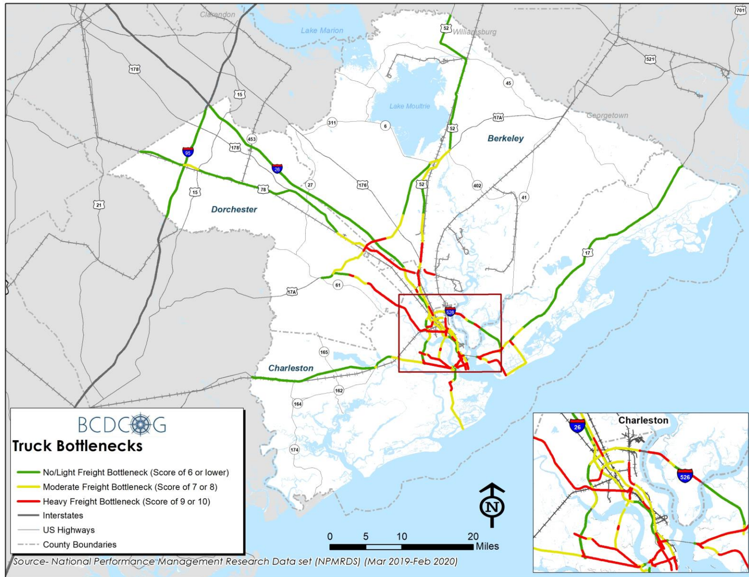
Figure 4-6: NPMRDS Truck Bottlenecks (2019-2020)
