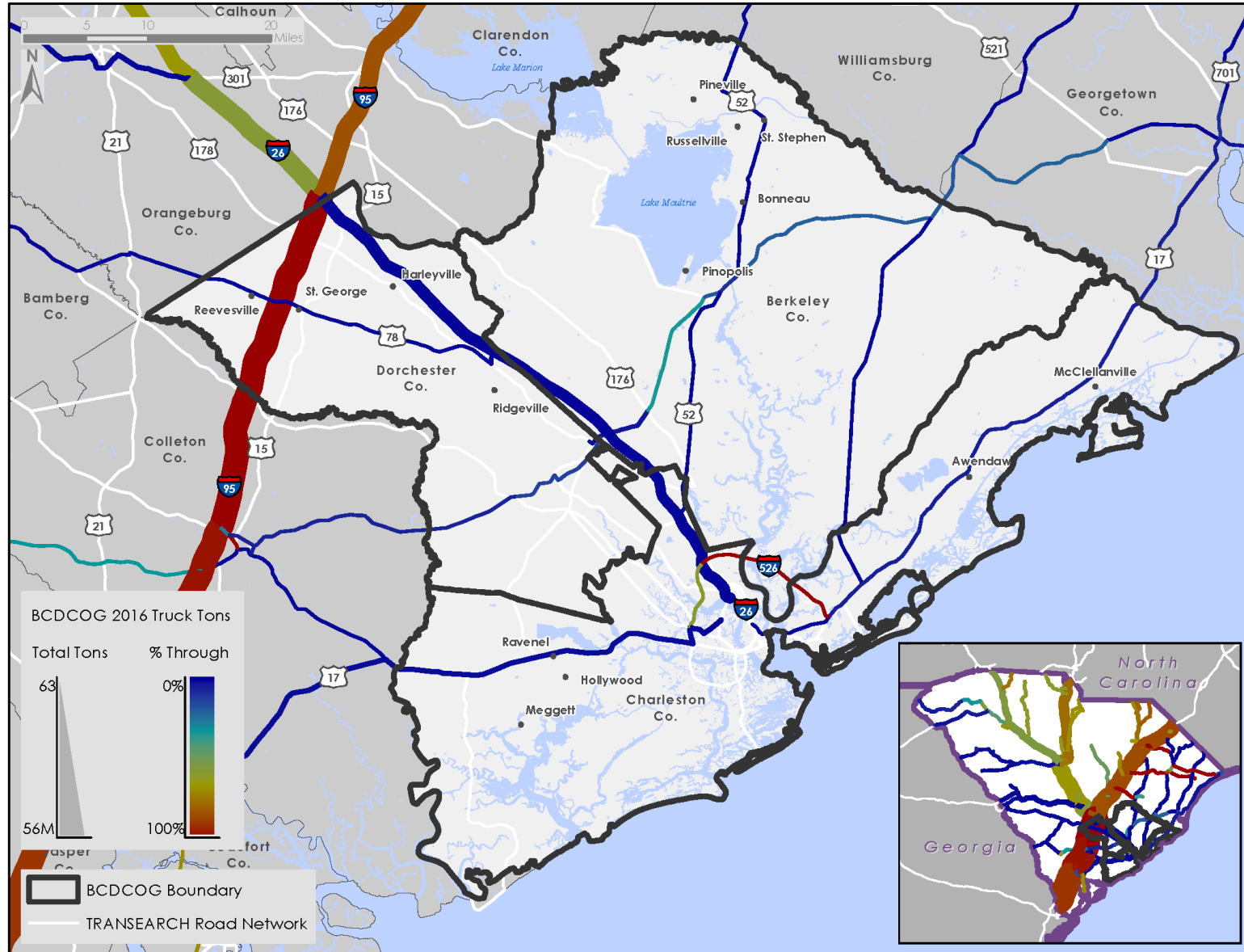
Figure 2-1: BCD Truck Tonnage Density and Percent Through Traffic, 2016
