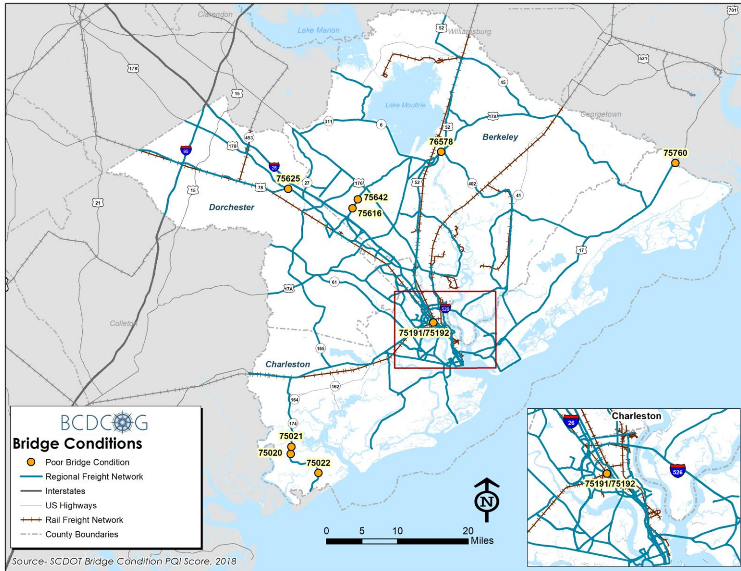
Figure 4-7: Freight Network Bridges in Poor Condition, 2018
